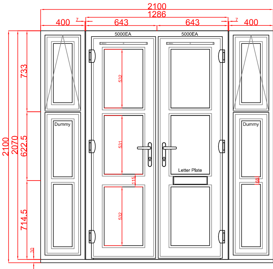
Frame type 1
