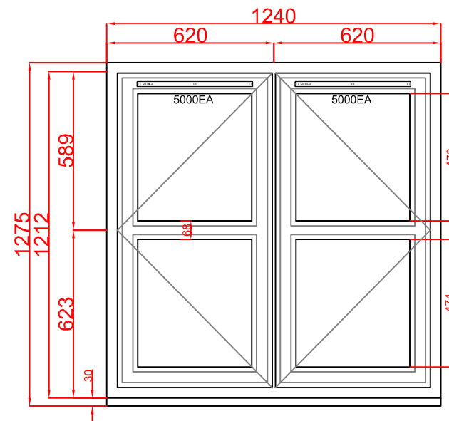
Frame type 3
