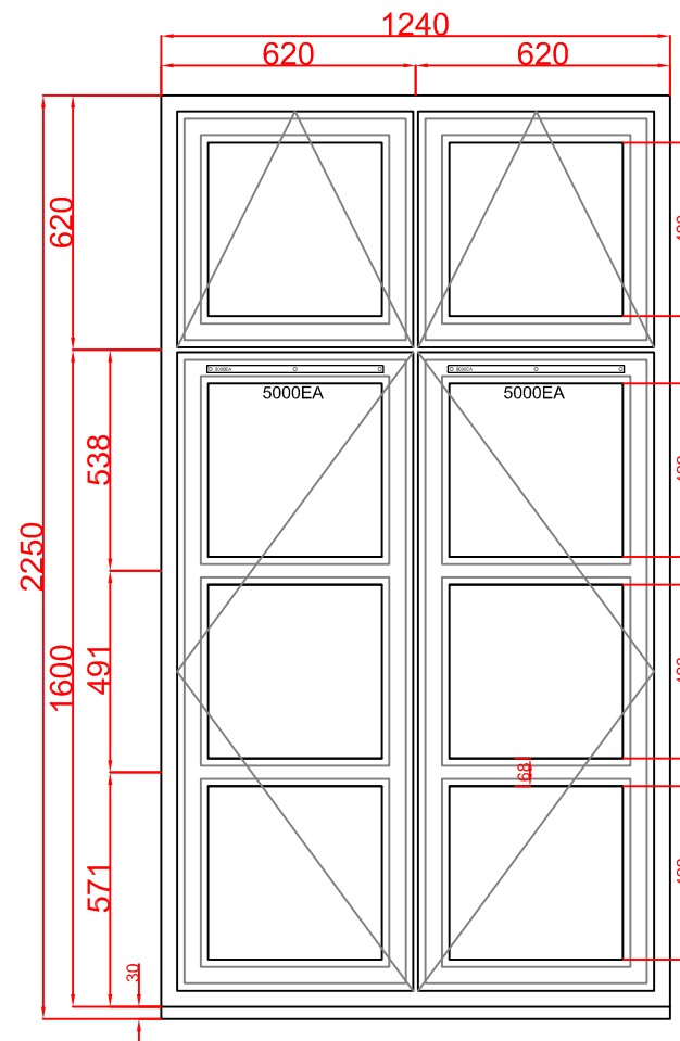
Frame type 2
