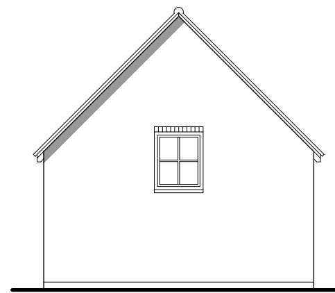
West elevation
