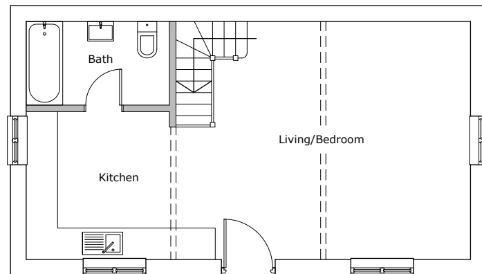
Floor plan
