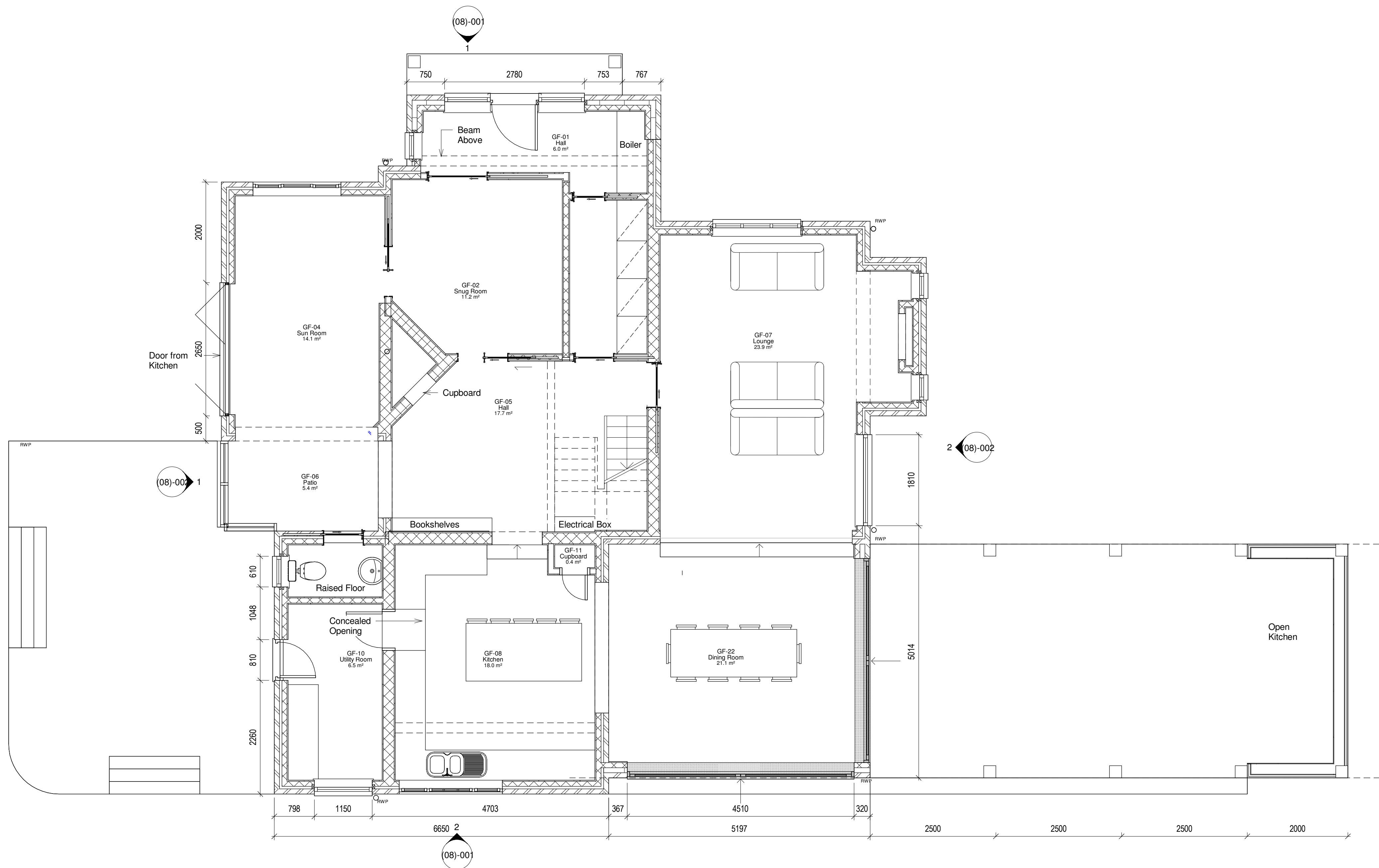
1 Ground Floor - Proposed Plan 1 : 50
