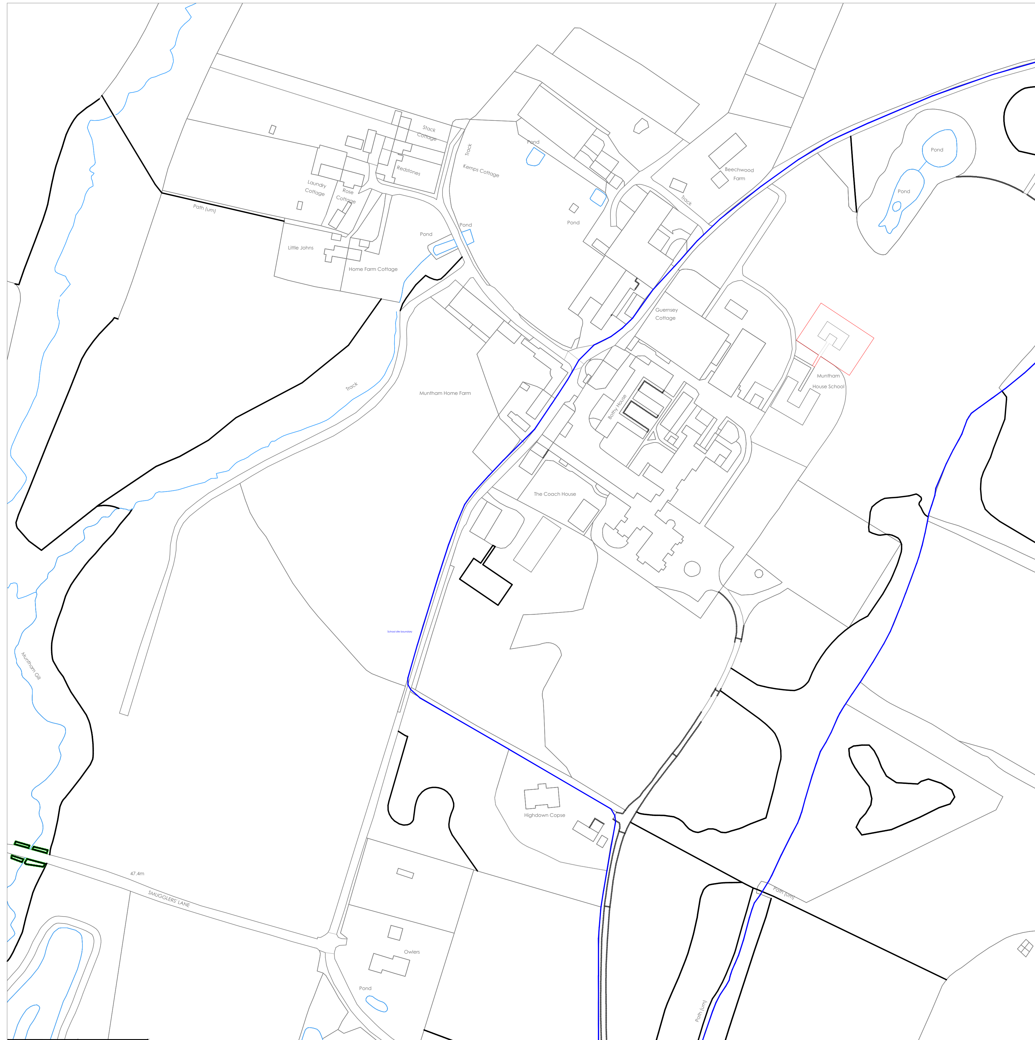
2 PROPOSED LOCATION PLAN 1:1250
