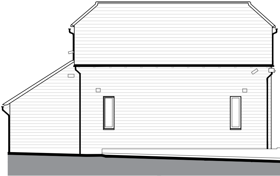
West Elevation
