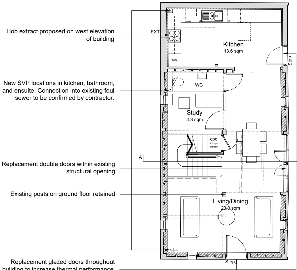
Proposed Ground Floor Plan The Granary 2-Bedroom 4-Person House 86.25 sqm / 928 sqft GIA [to finishes] 2.0sqm storage provided where shown [2.0sqm required]
