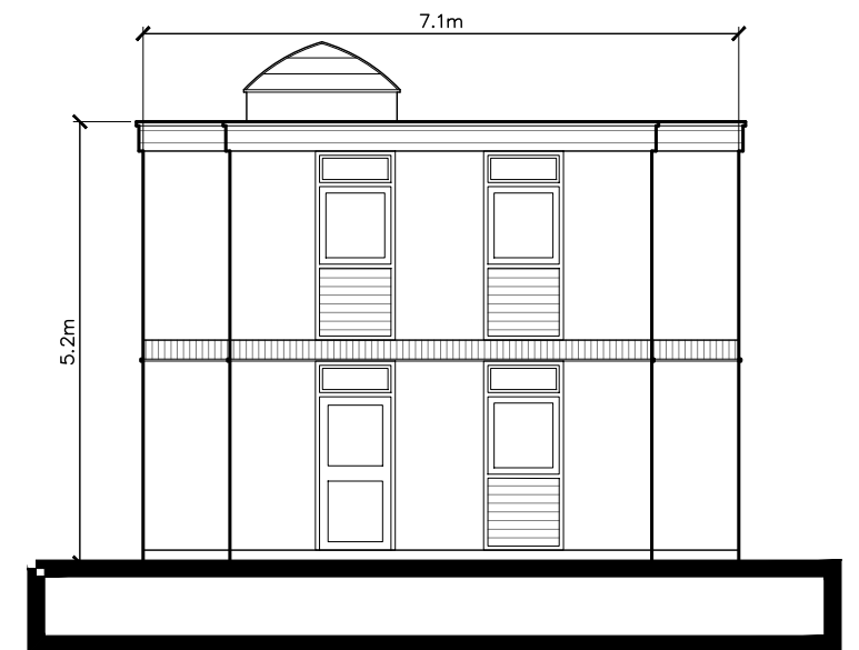
North Elevation 1:100
