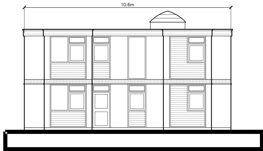
East Elevation 1:100
