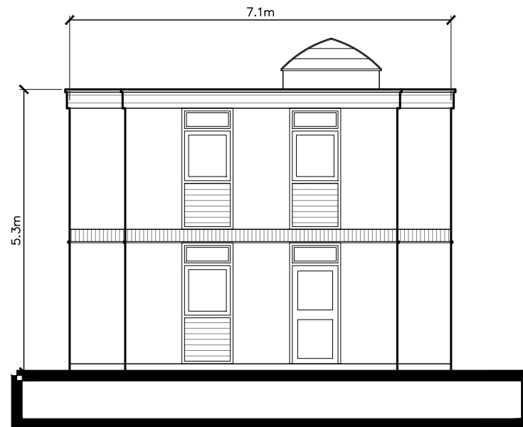
South Elevation 1:100
