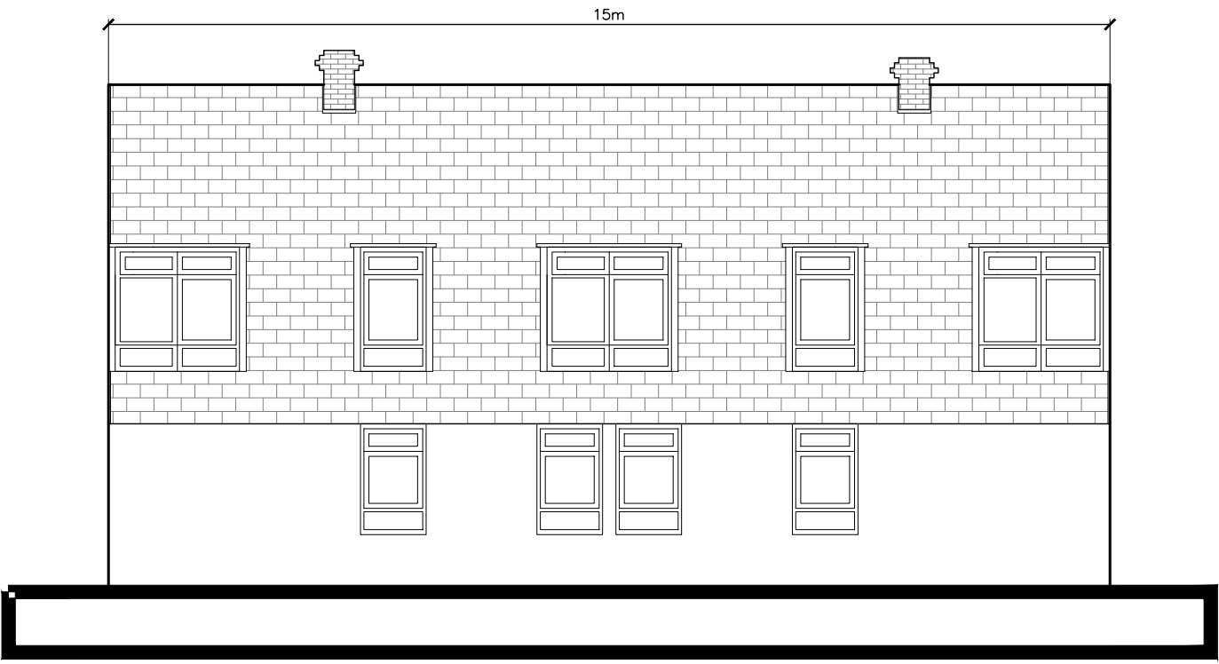
South Elevation 1:100
