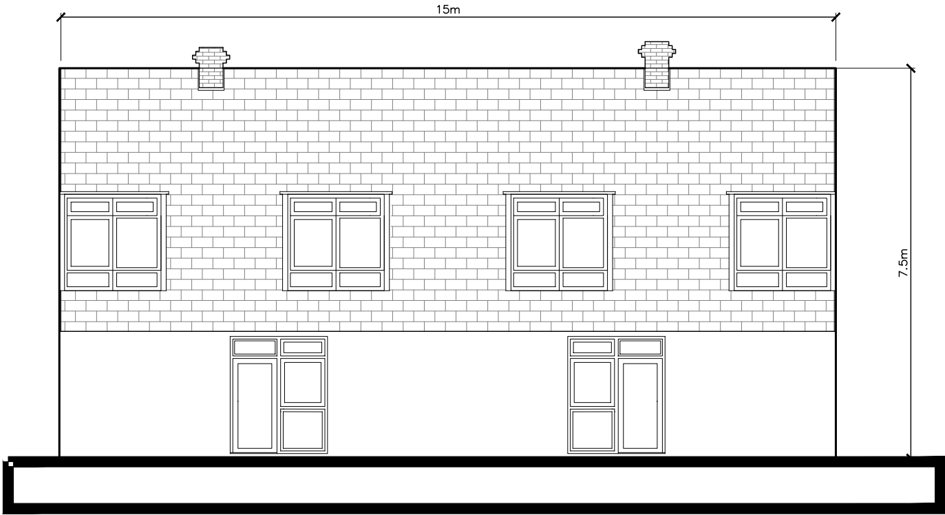
North elevation at 1:100
