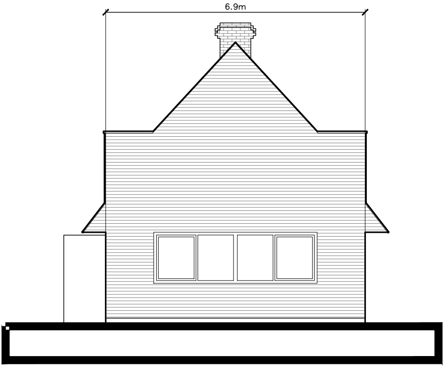
West Elevation at 1:100
