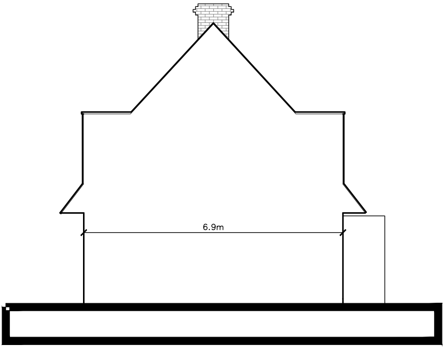
East Elevation 1:100
