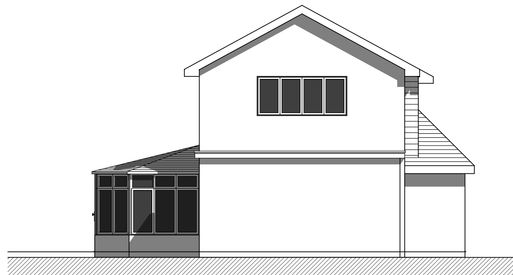
PR SIDE ELEVATION - 1:100 39 Saltings Way, Upper Beeding, BN44 3JH
