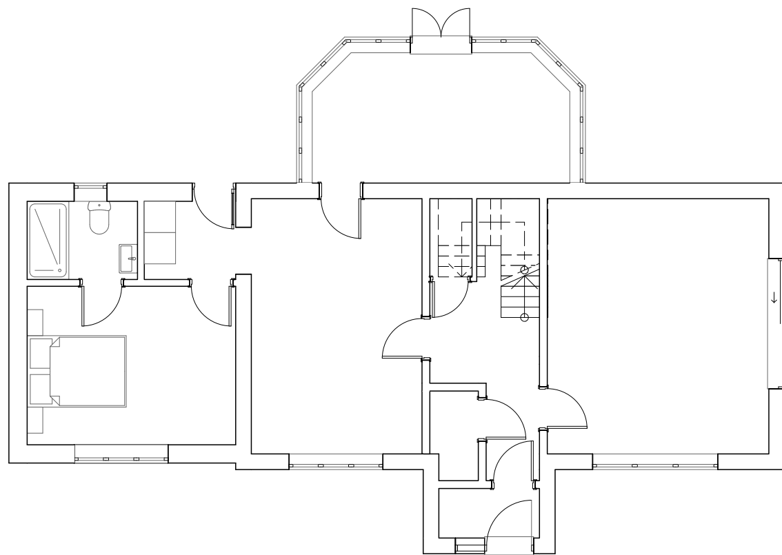
PR GROUND FLOOR - 1:100 39 Saltings Way, Upper Beeding, BN44 3JH
