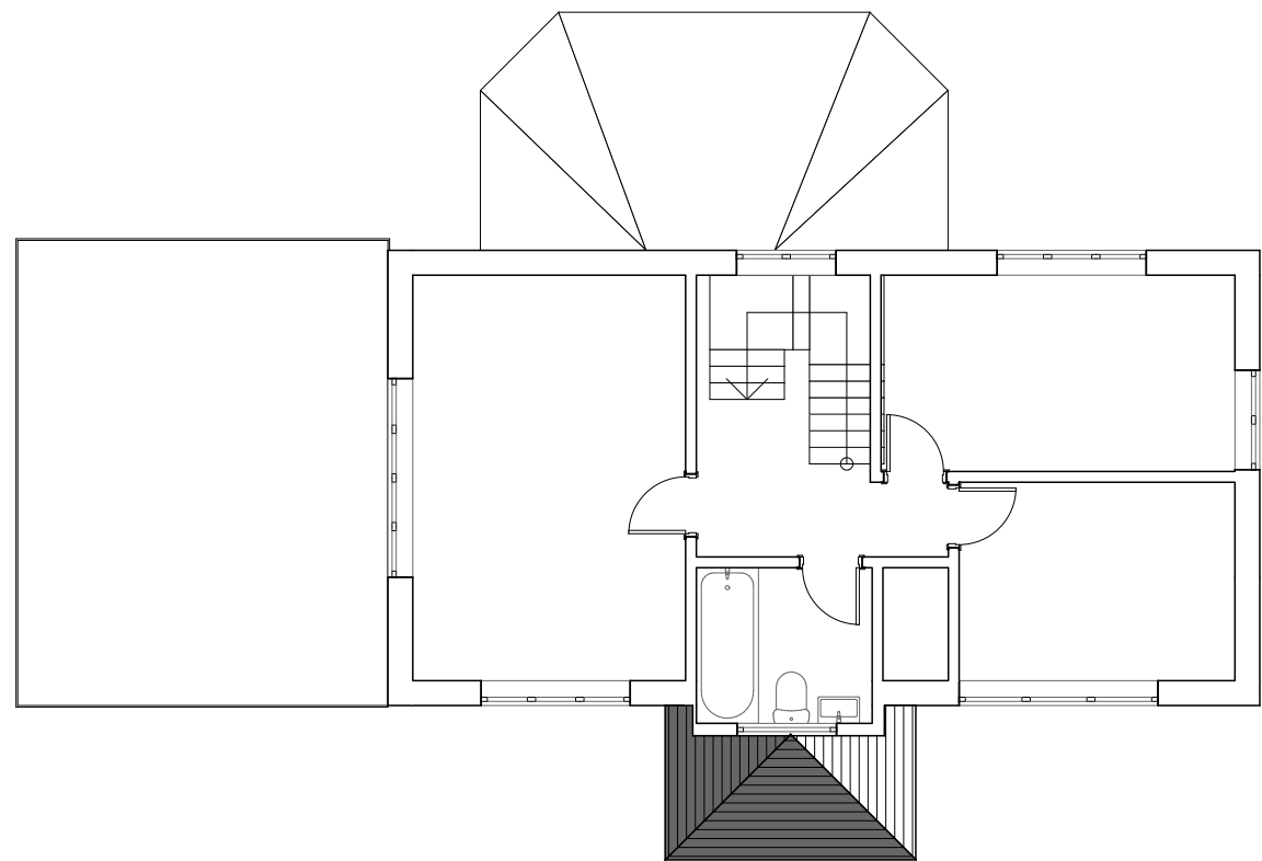
PR FIRST FLOOR - 1:100 39 Saltings Way, Upper Beeding, BN44 3JH
