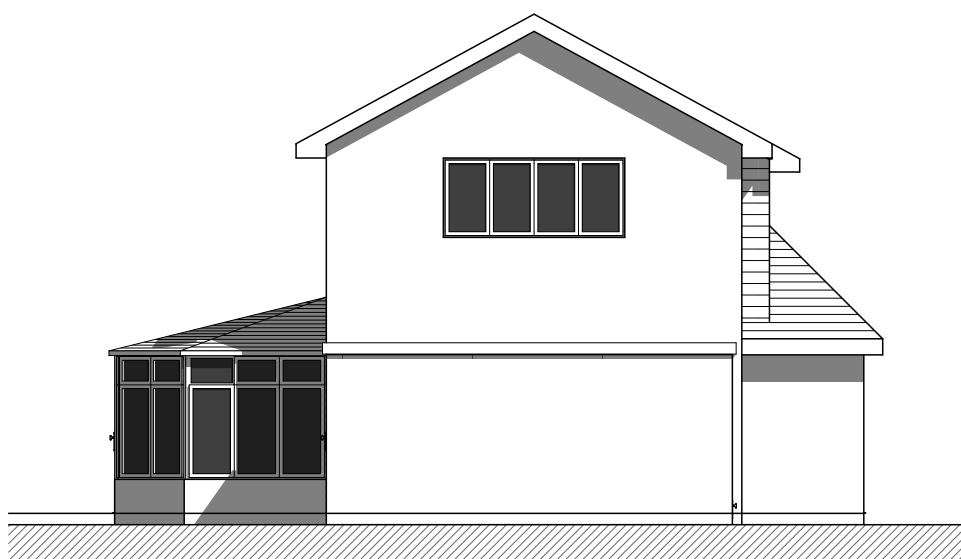
EX SIDE ELEVATION - 1:100 39 Saltings Way, Upper Beeding, BN44 3JH
