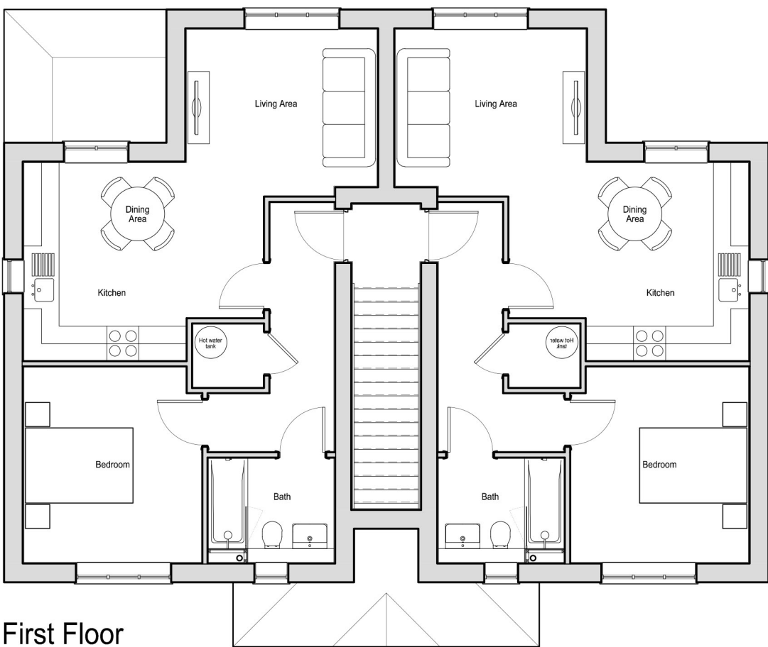
First Floor
