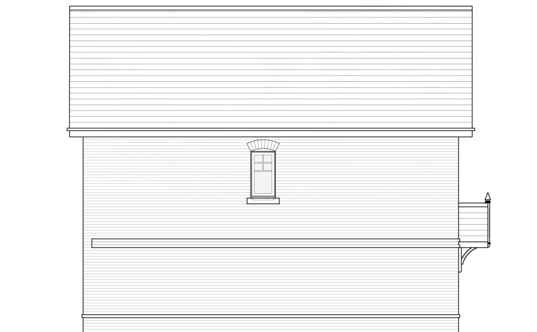
Side Elevation
