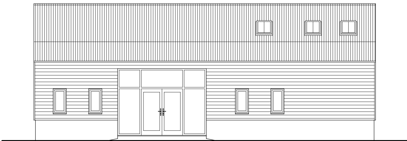
PROPOSED REAR (SOUTH) ELEVATION
