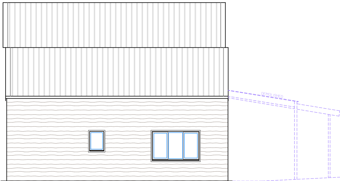
BARN A EAST ELEVATION
