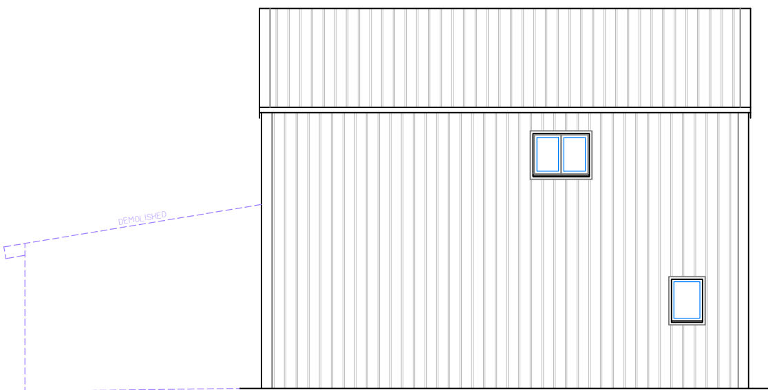
BARN A WEST ELEVATION
