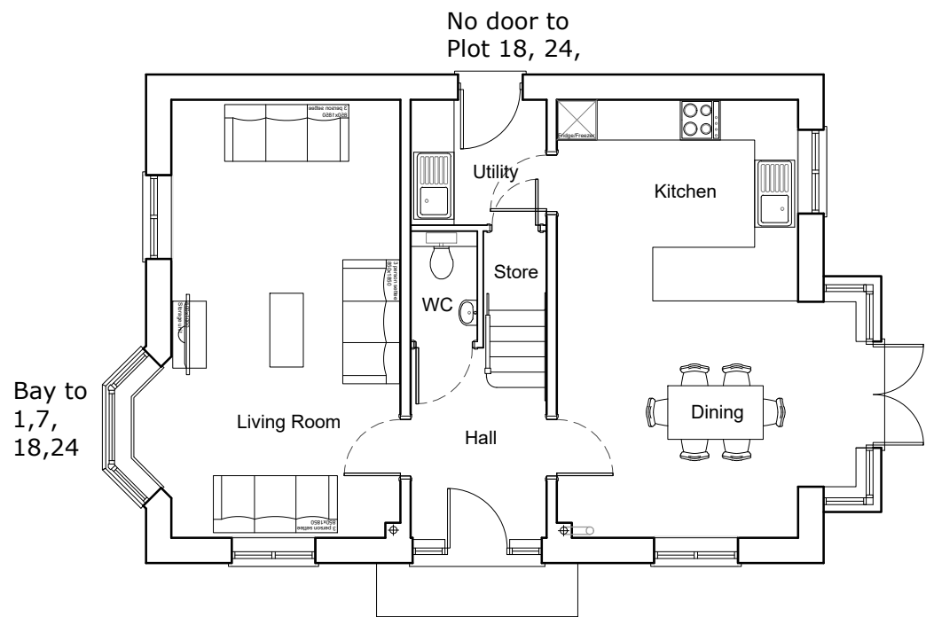
GROUND FLOOR Plots 1, 7, 18, 24
