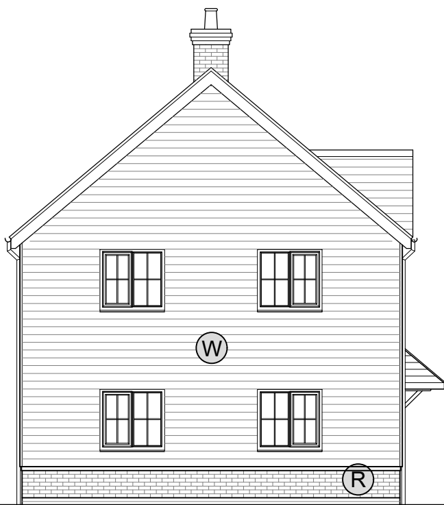
SIDE ELEVATION
