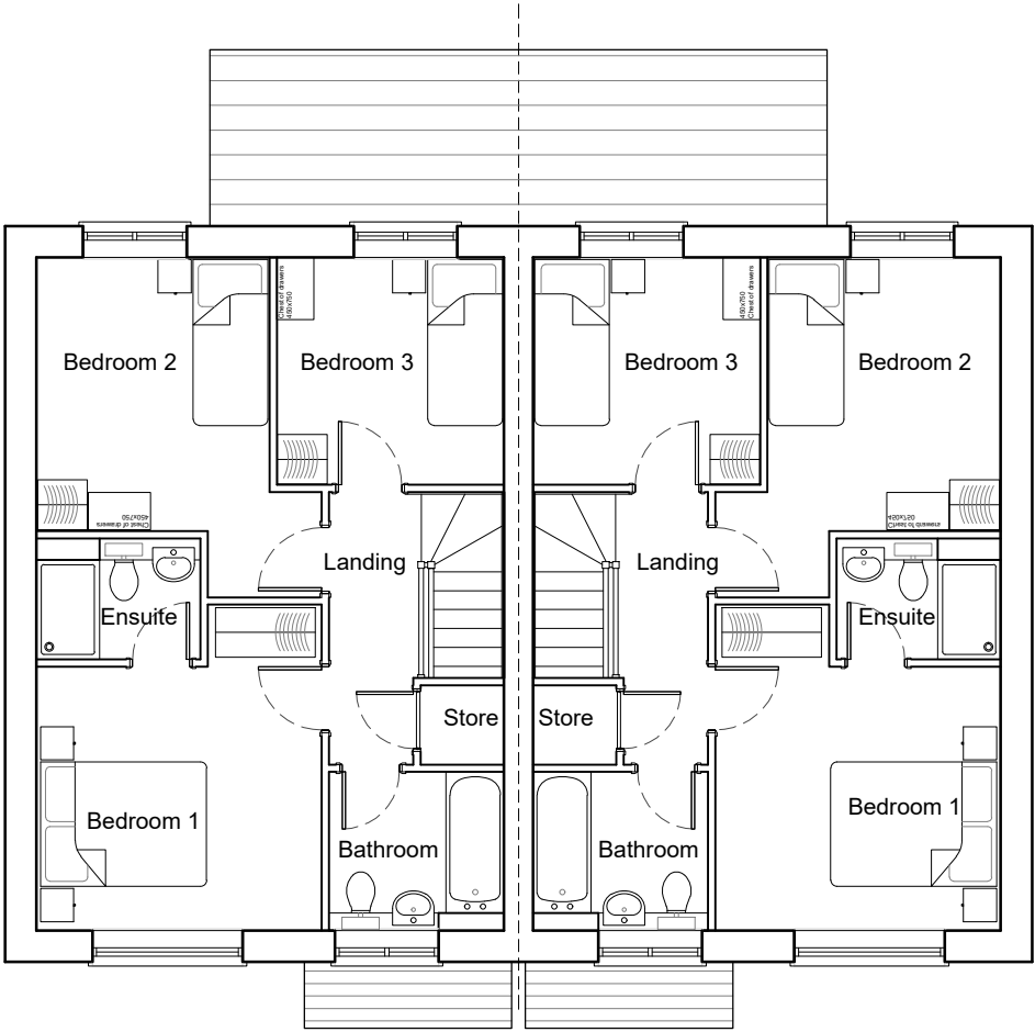
FIRST FLOOR
