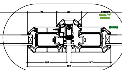
DETAIL 8
