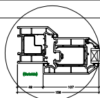
DETAIL 7
