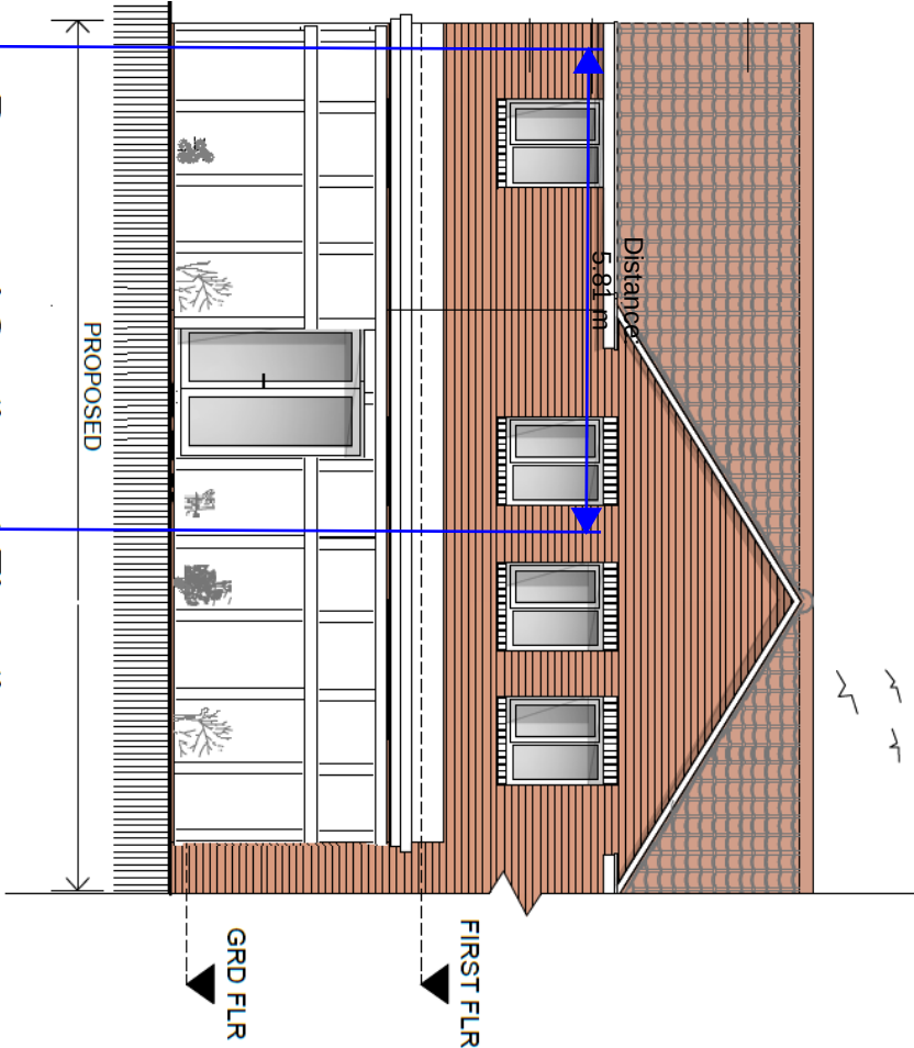
Proposed Southwest Elevation
