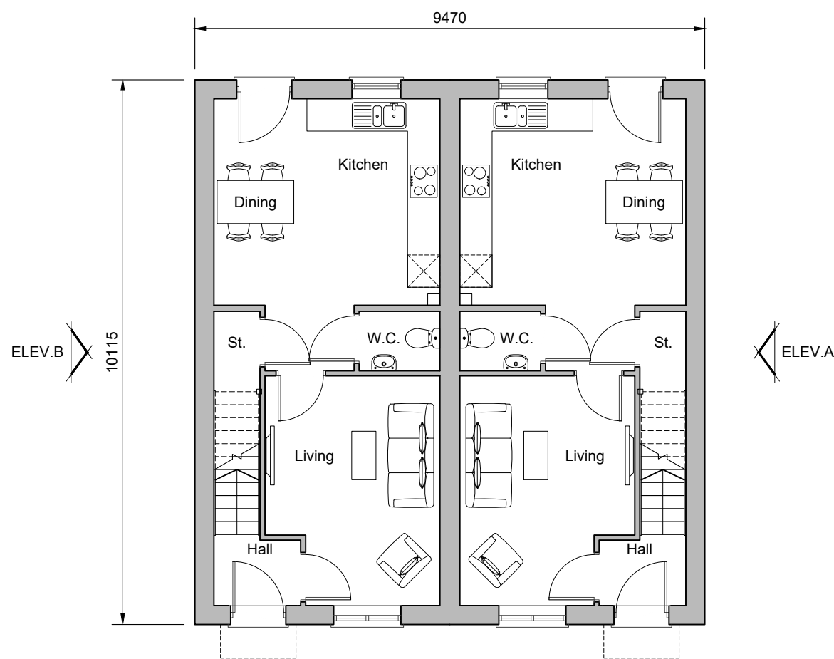
Ground Floor Plan Plots 51-52 & 60-61
