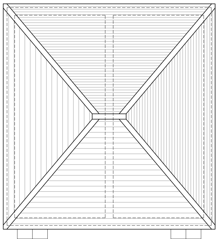
Roof Plan
