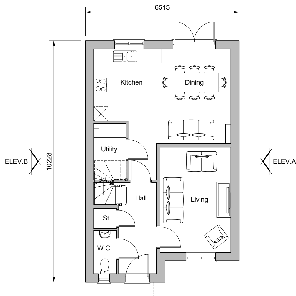
Ground Floor Plan Plot 28
