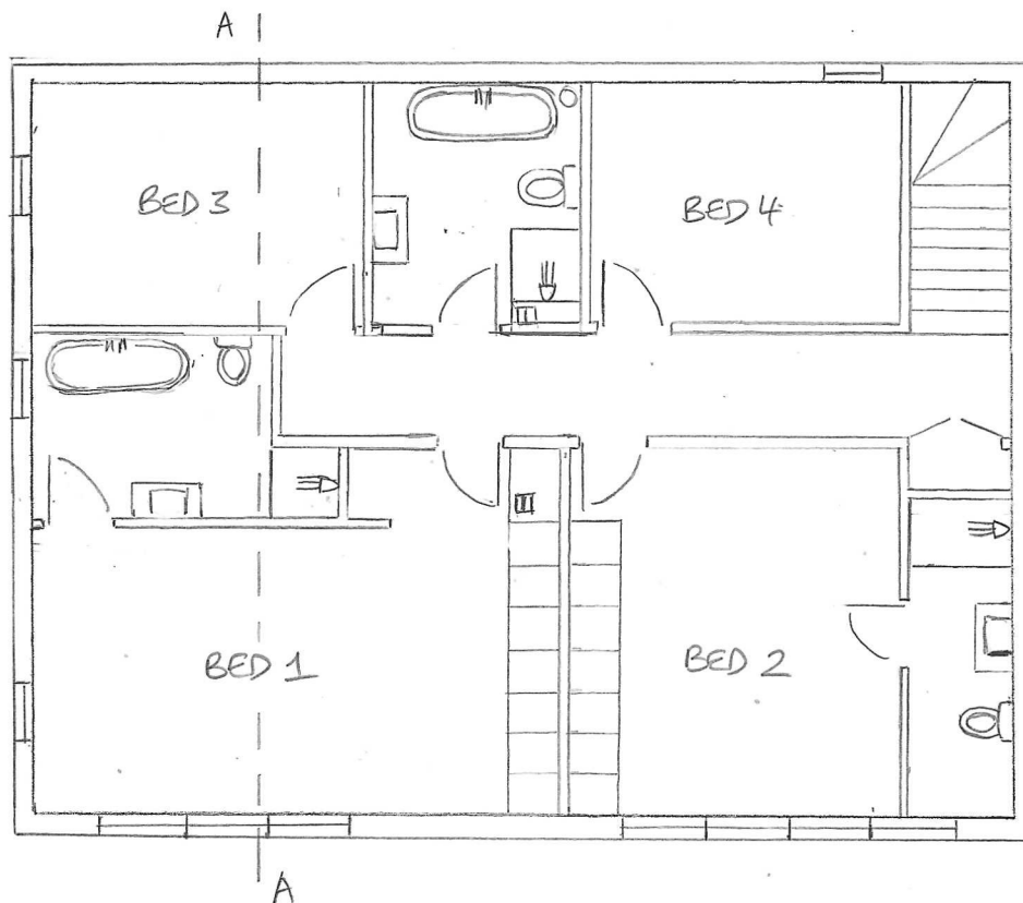
PROPOSED FLOOR PLAN - 1 ST FLOOR
