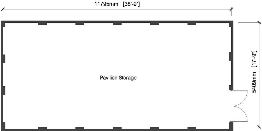
Floor Plan
