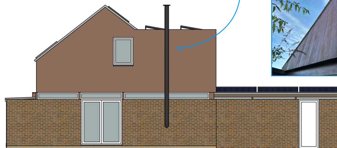
SOUTHERN ELEVATION
