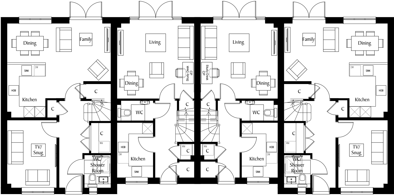
M3.4 Plot 185 M2.2 Plot 184 M2.2 Plot 183 M3.4 Plot 182 Ground Floor
