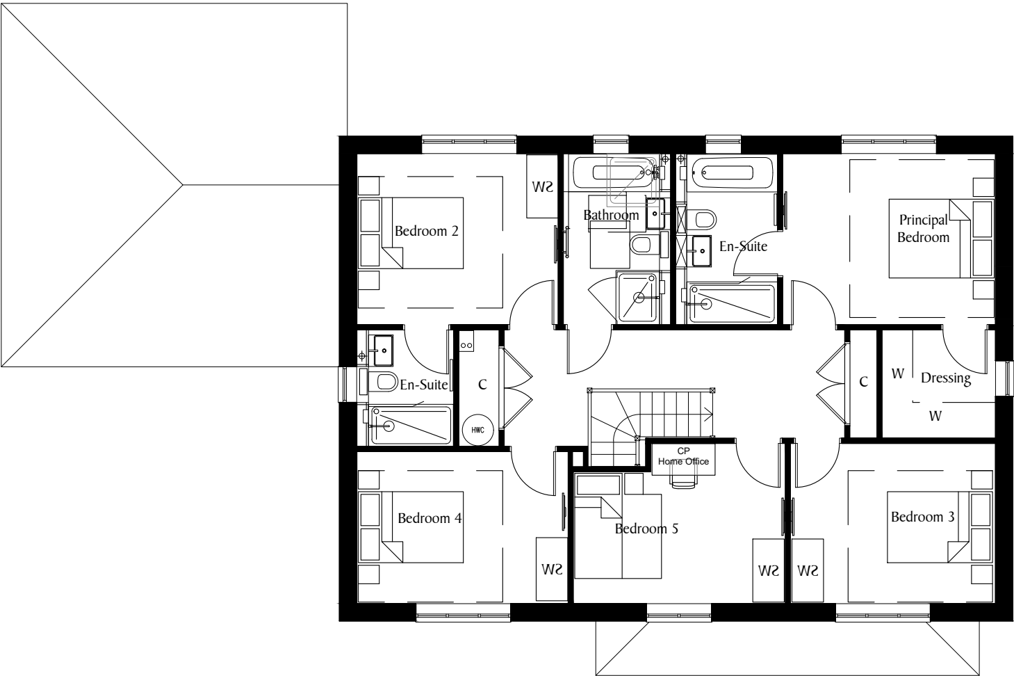
First Floor
