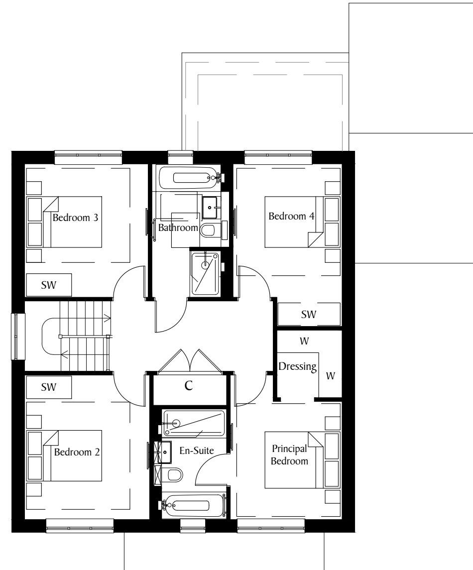
First Floor
