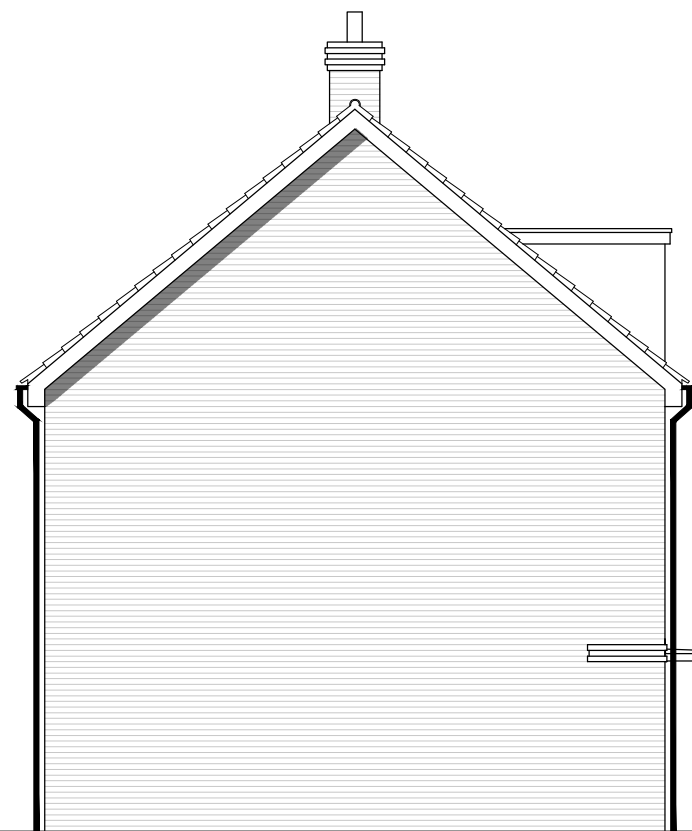
Side Elevation
