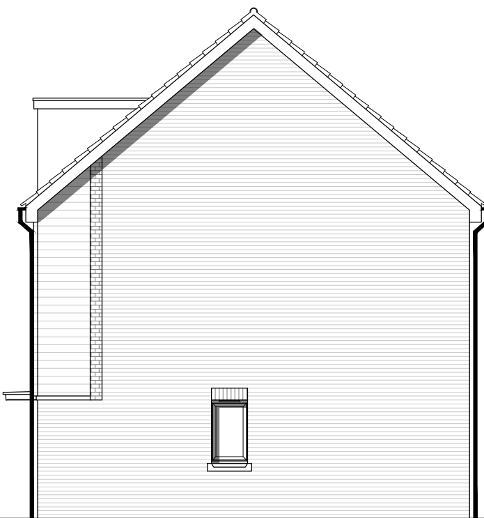
Side Elevation
