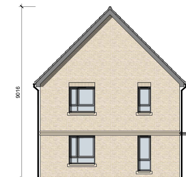
Front Elevation
