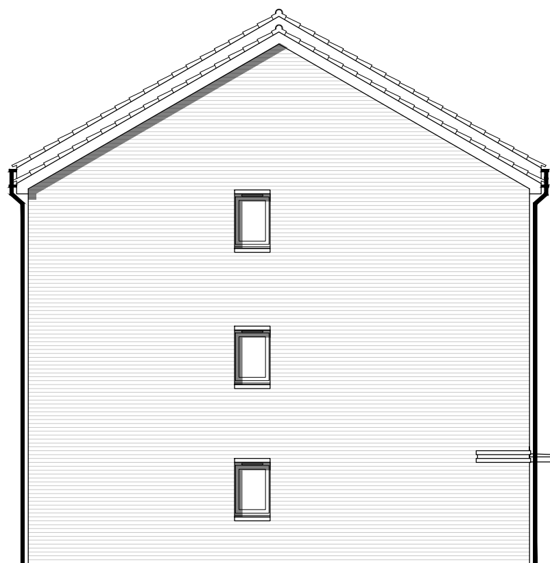
Side Elevation
