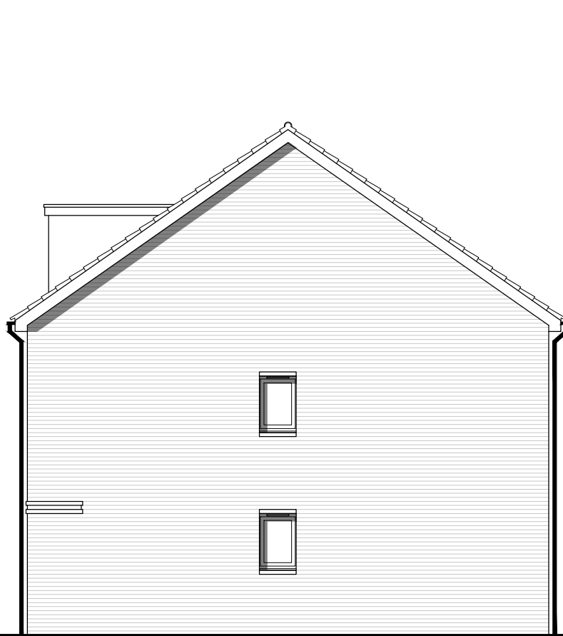
Side Elevation
