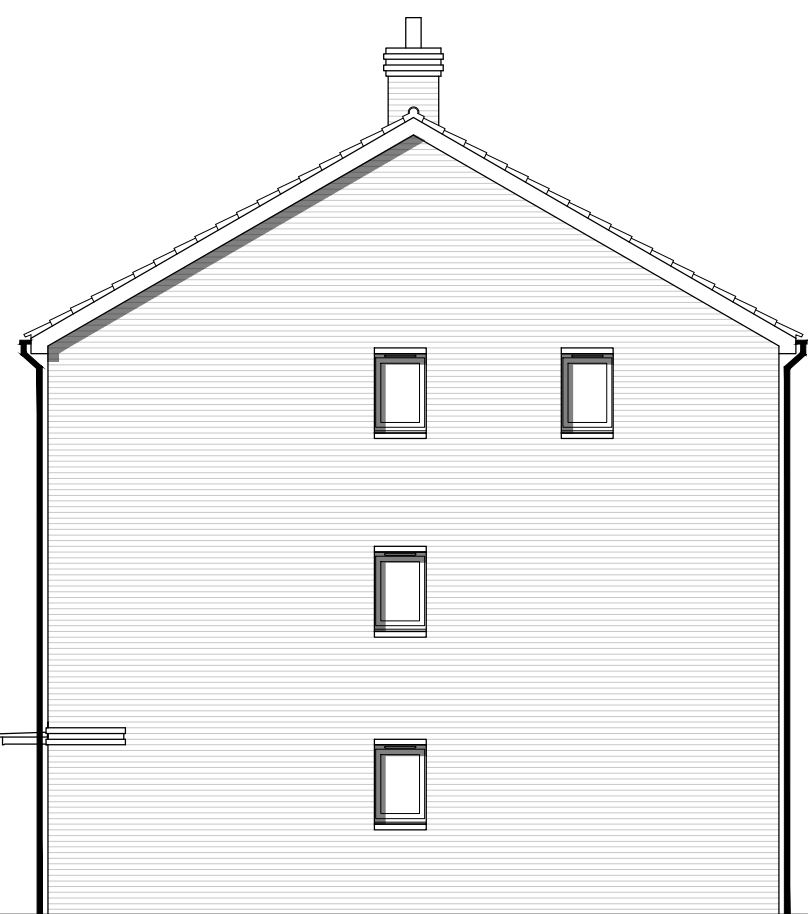
Side Elevation
