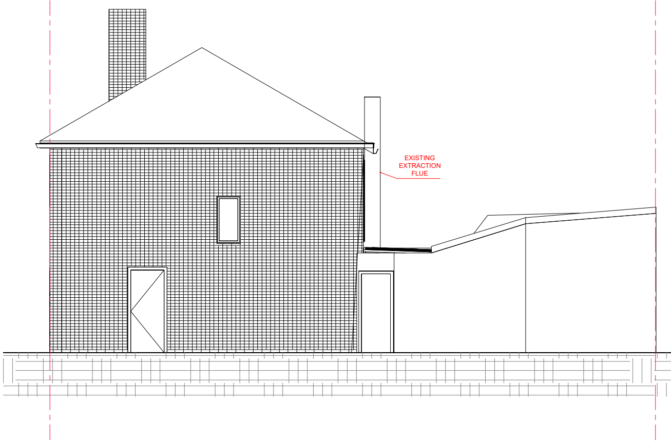
Existing Side Elevation (North)
