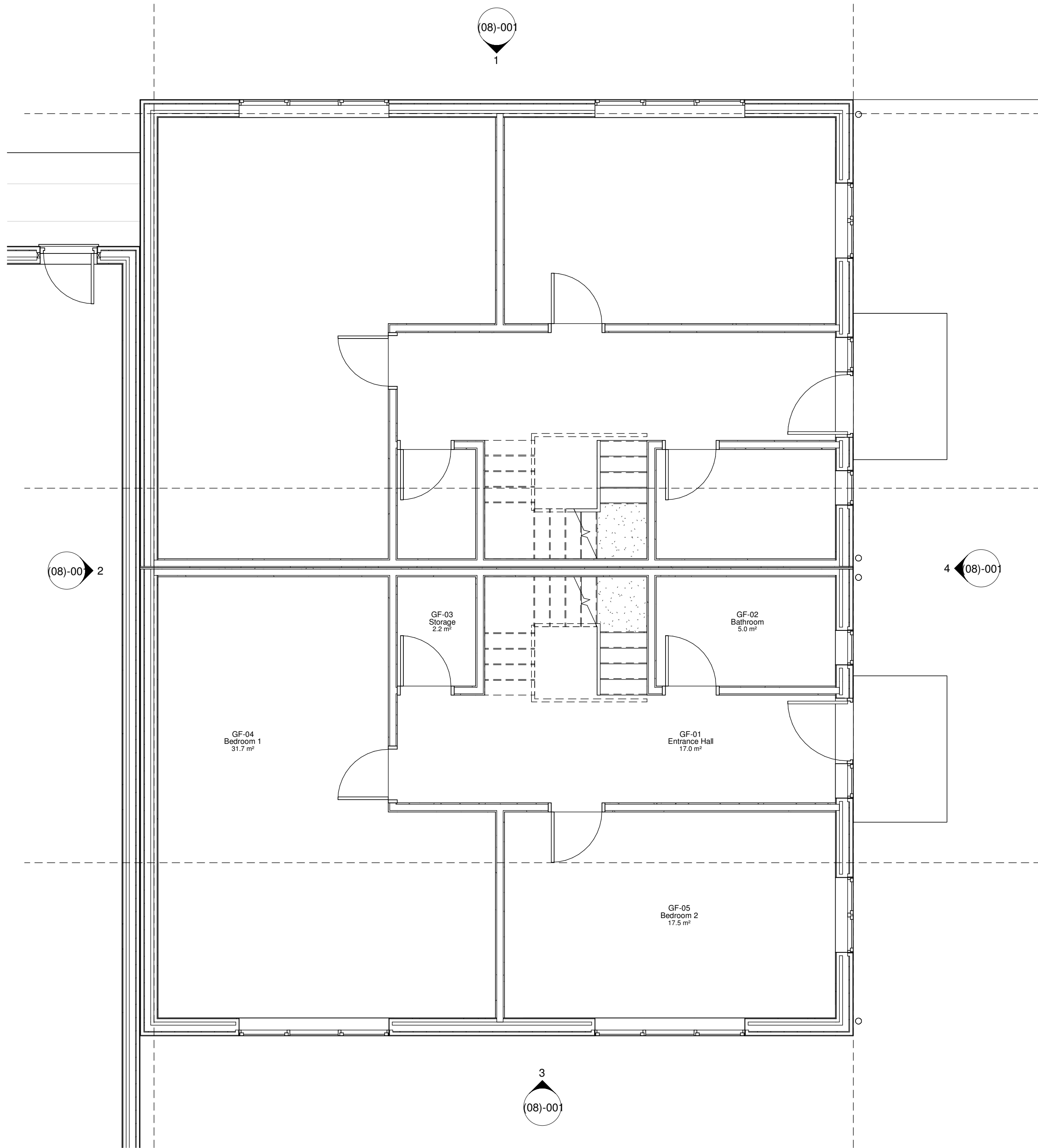
1 Ground Floor - Proposed Plan 1 : 50
