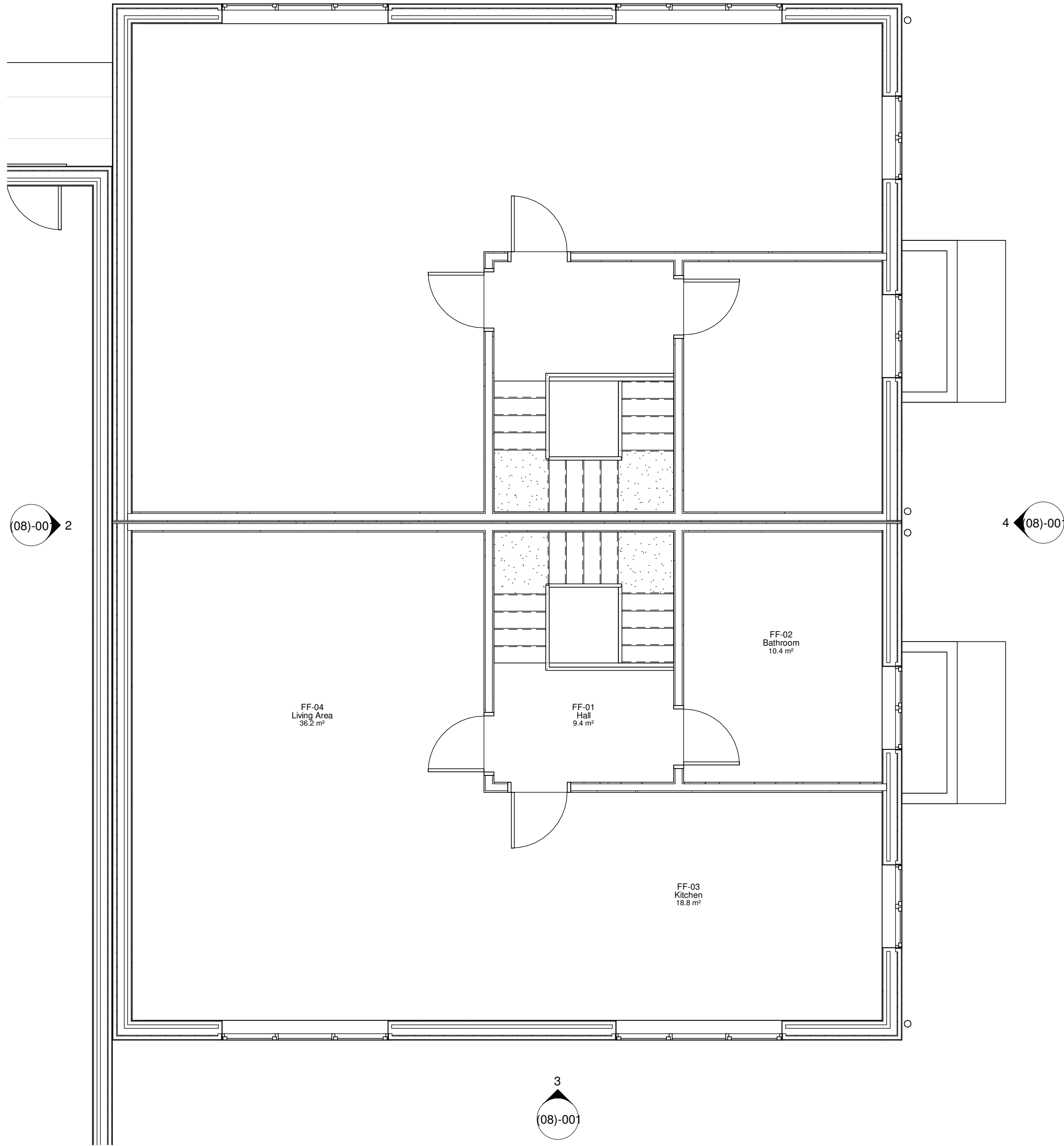
3 First Floor - Proposed Plan 1 : 50
