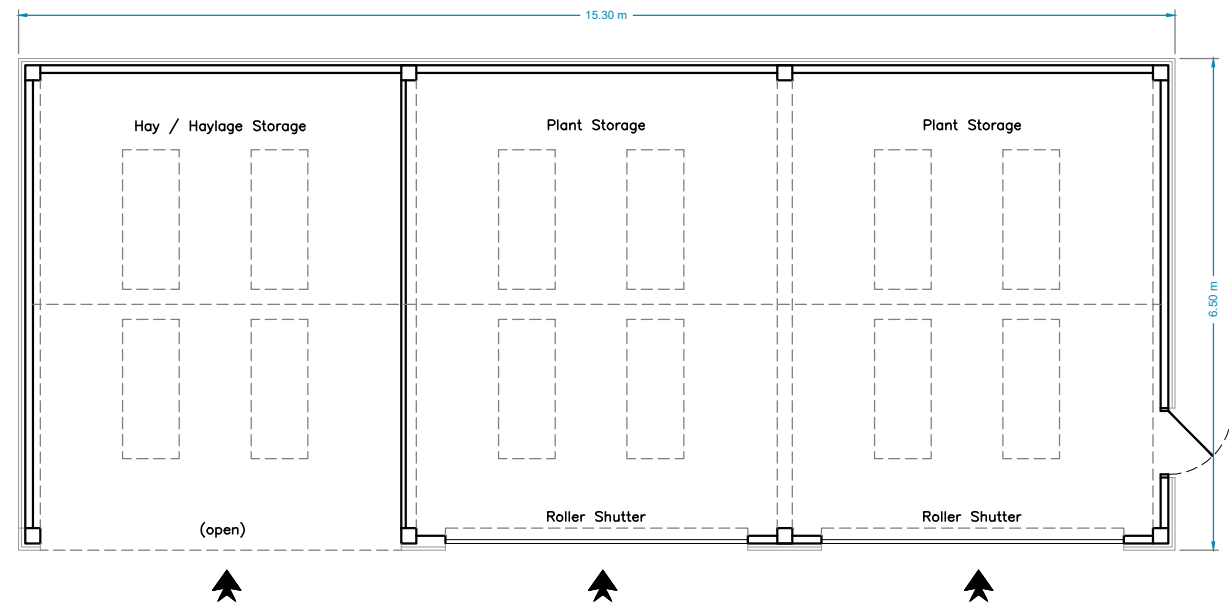
Ground Floor G.I.A. 91m 2
