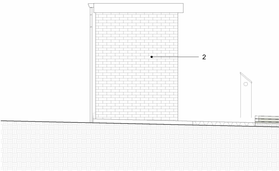
CYCLE STORE ELEVATION C 1 : 50
