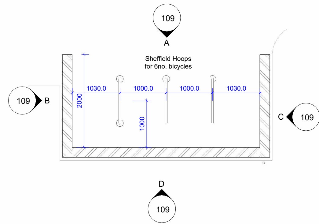
CYCLE STORE PLAN 1 : 50
