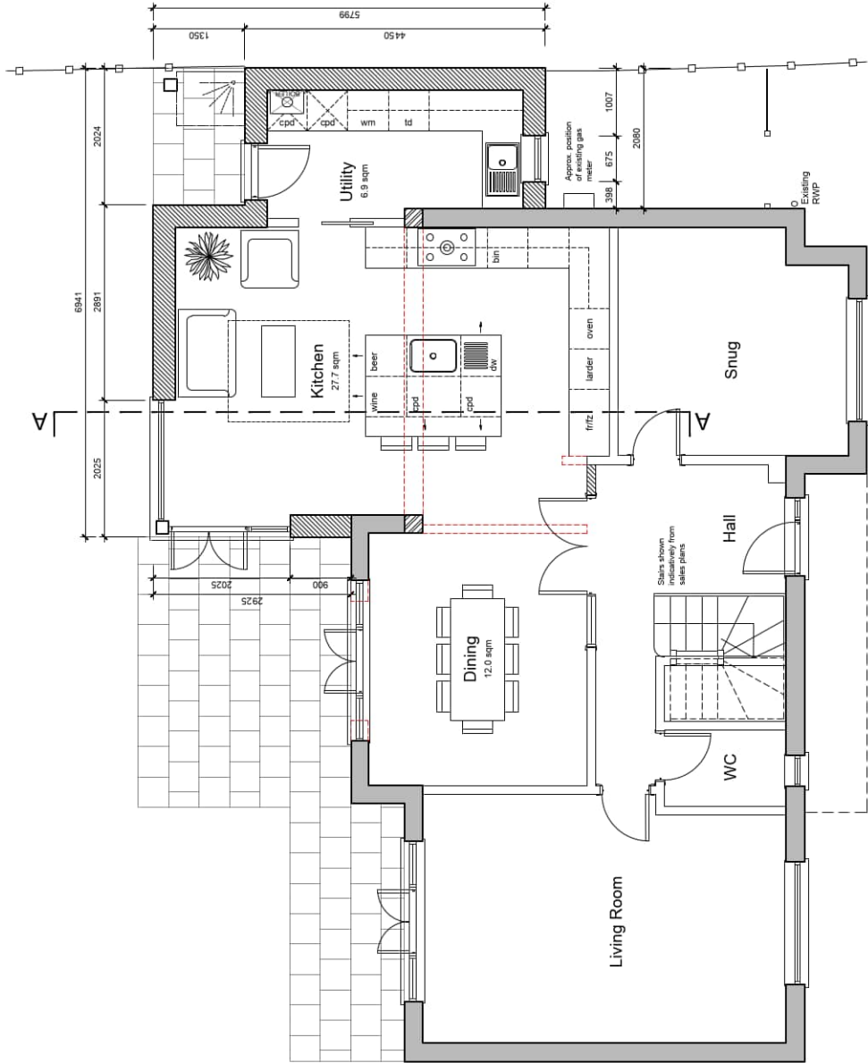
Proposed Ground Floor Plan 1:100 Additional GIA 21.58 sqm / 232sqft
