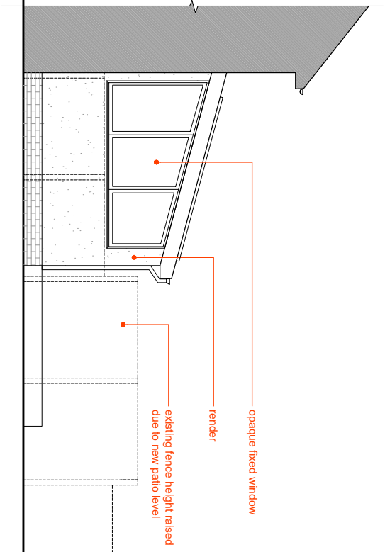
side elevation
