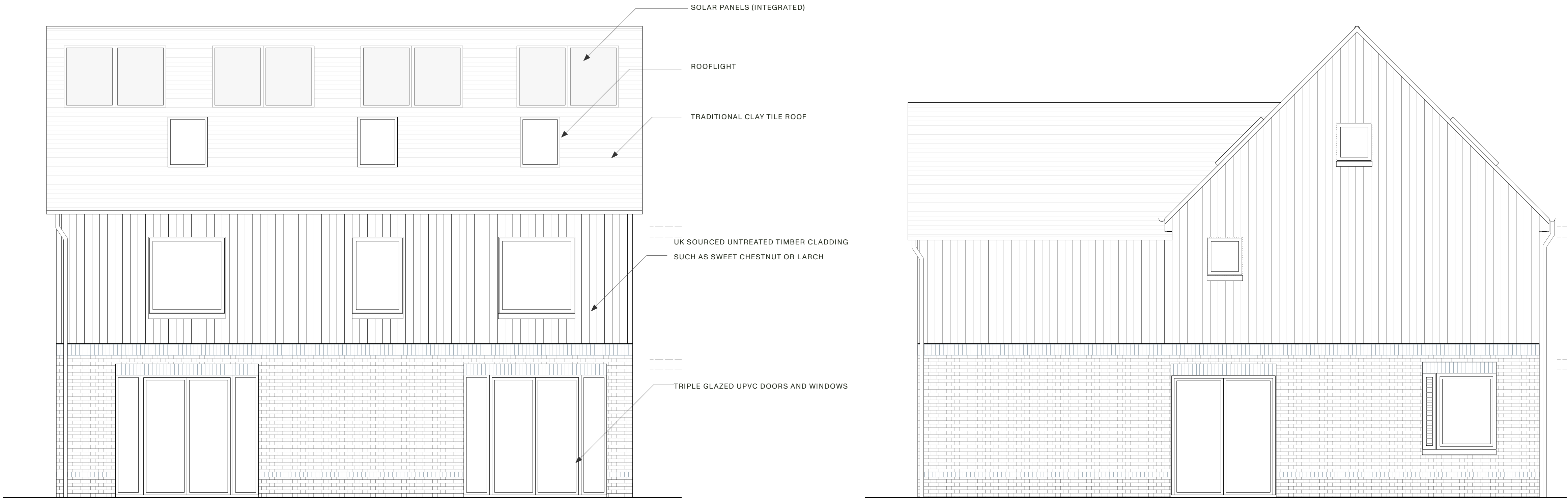
AS PROPOSED REAR ELEVATION (WEST)
