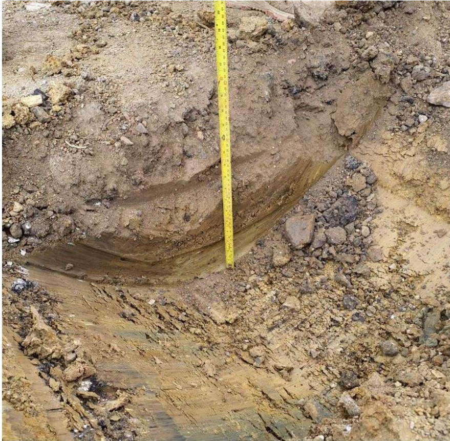
Inspection pit excavated 450mm into the formation level, indicating made ground was present in the formation level soils
