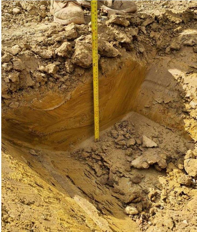
Inspection pit excavated 400mm into formation level of Plot 13
