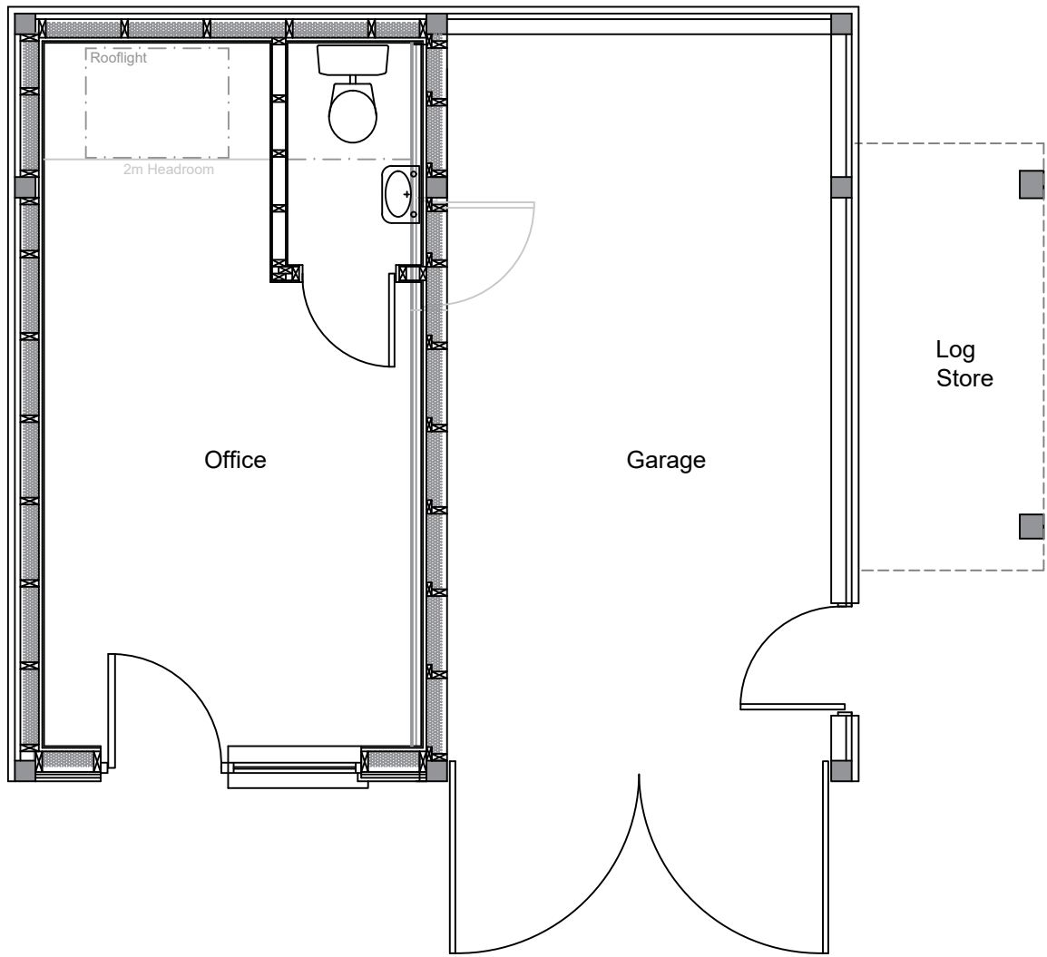
Proposed Layout (Scale 1:50)
