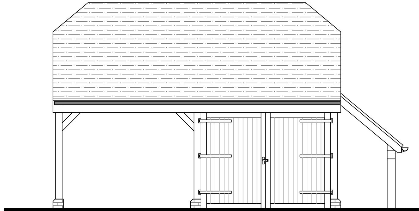
Existing Front Elevation (Scale 1:50)
