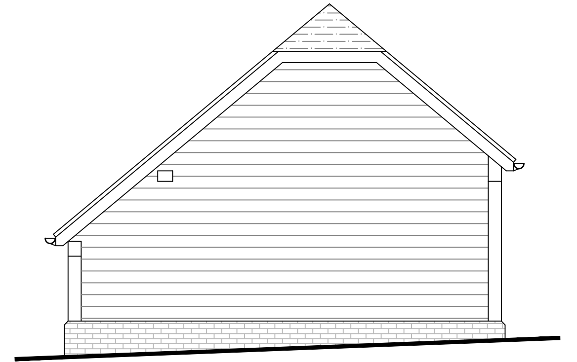
Existing Side Elevation (Scale 1:50)
