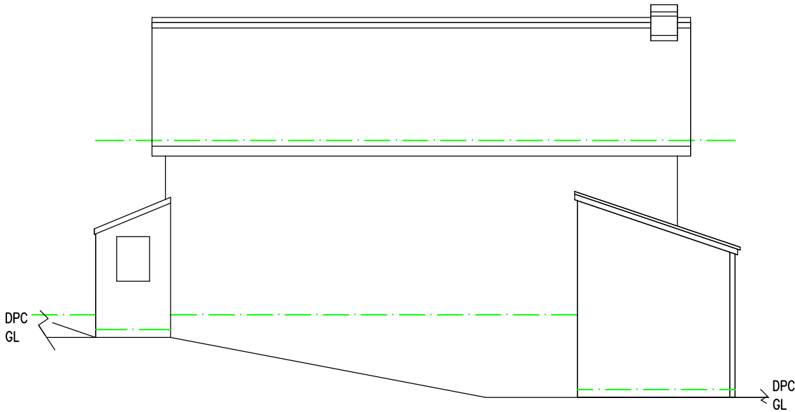
Existing Rear Elevation (West)
