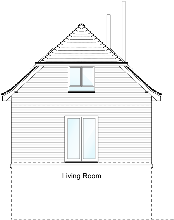
West Elevation [Side]
