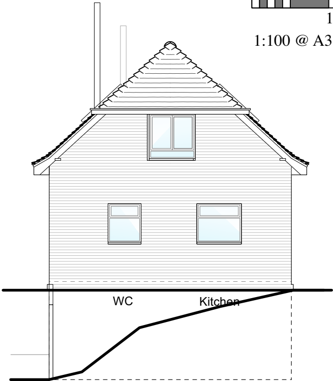
Plant Room East Elevation [Side]
