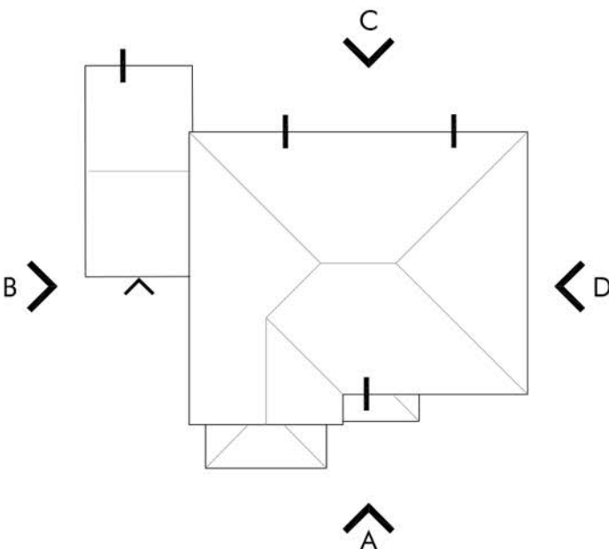
ROOF PLAN 1:200
