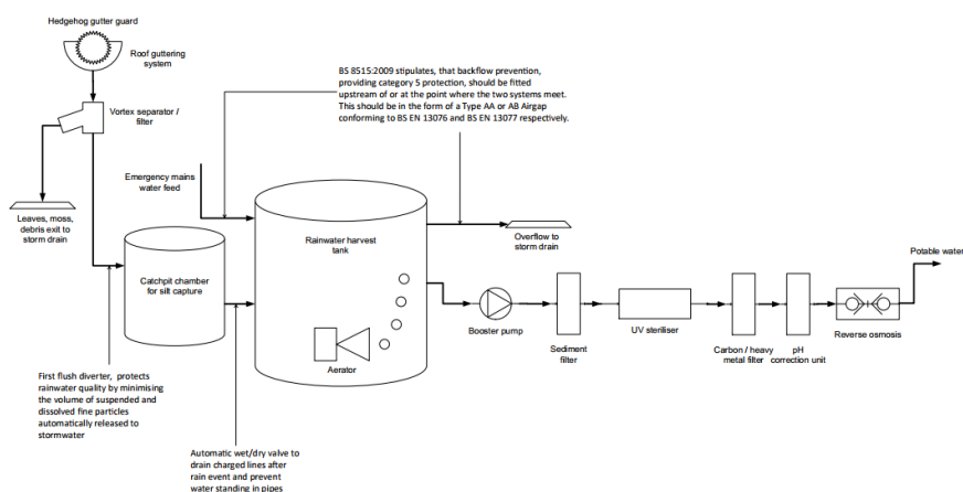
Fig. 6 Schematic view of treatment system
