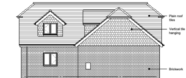
PROPOSED SIDE ELEVATION (North West)
