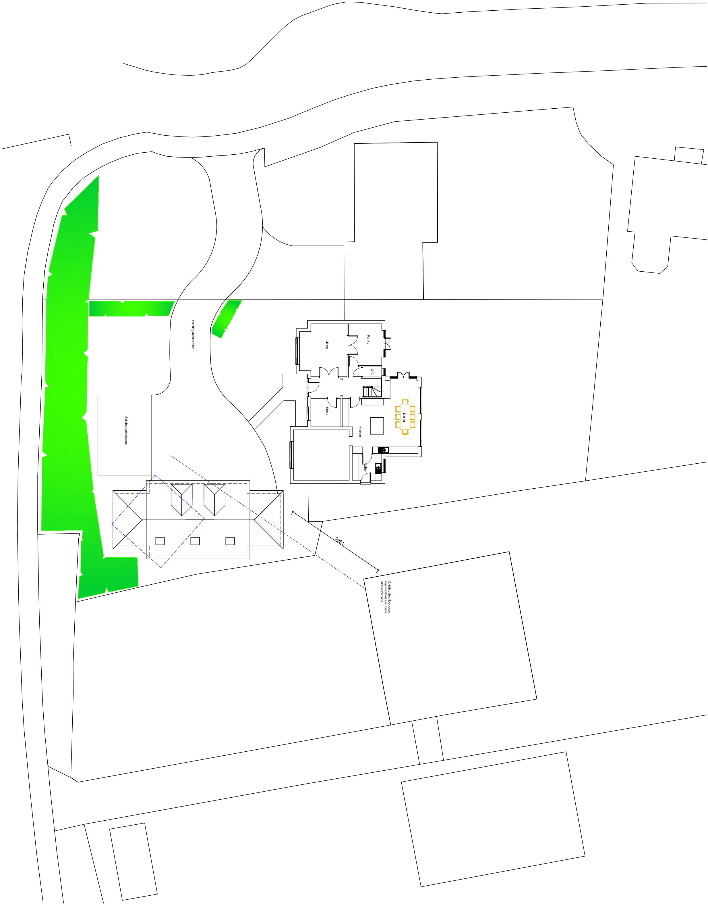
Location Plan 1:1250
