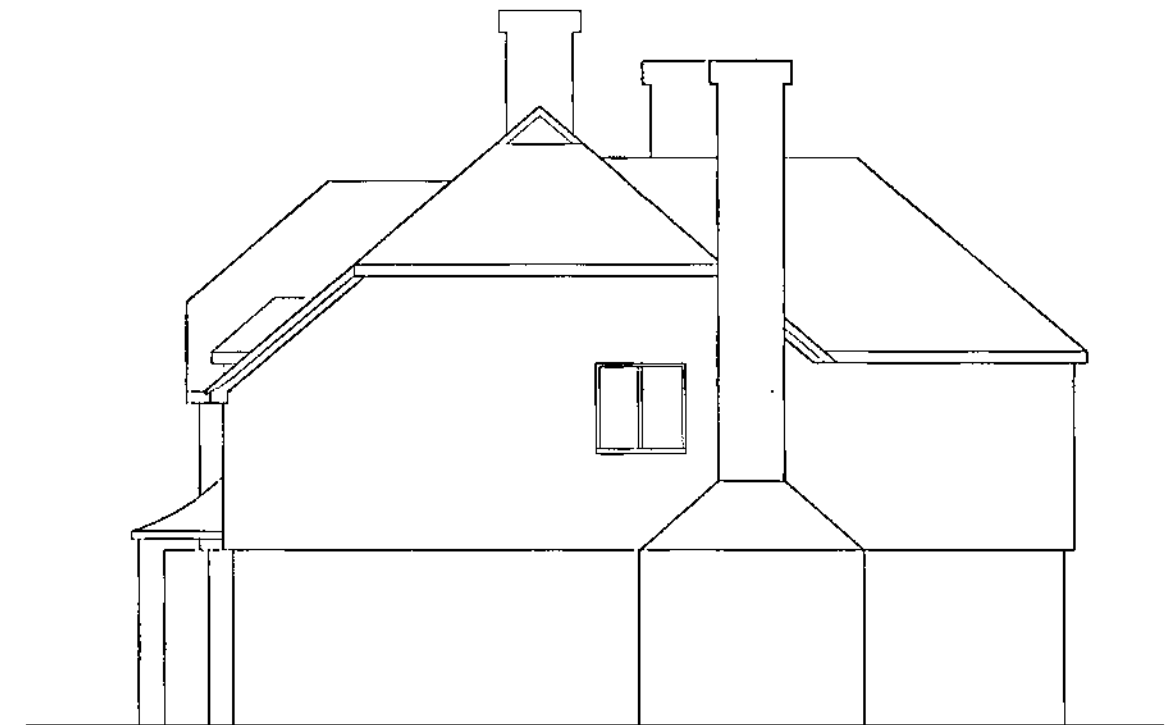
NORTH ELEVATION 1:100
