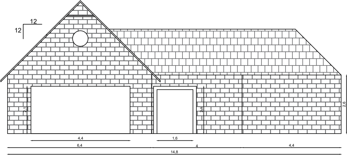
ELEVATION Scale 1: 100
