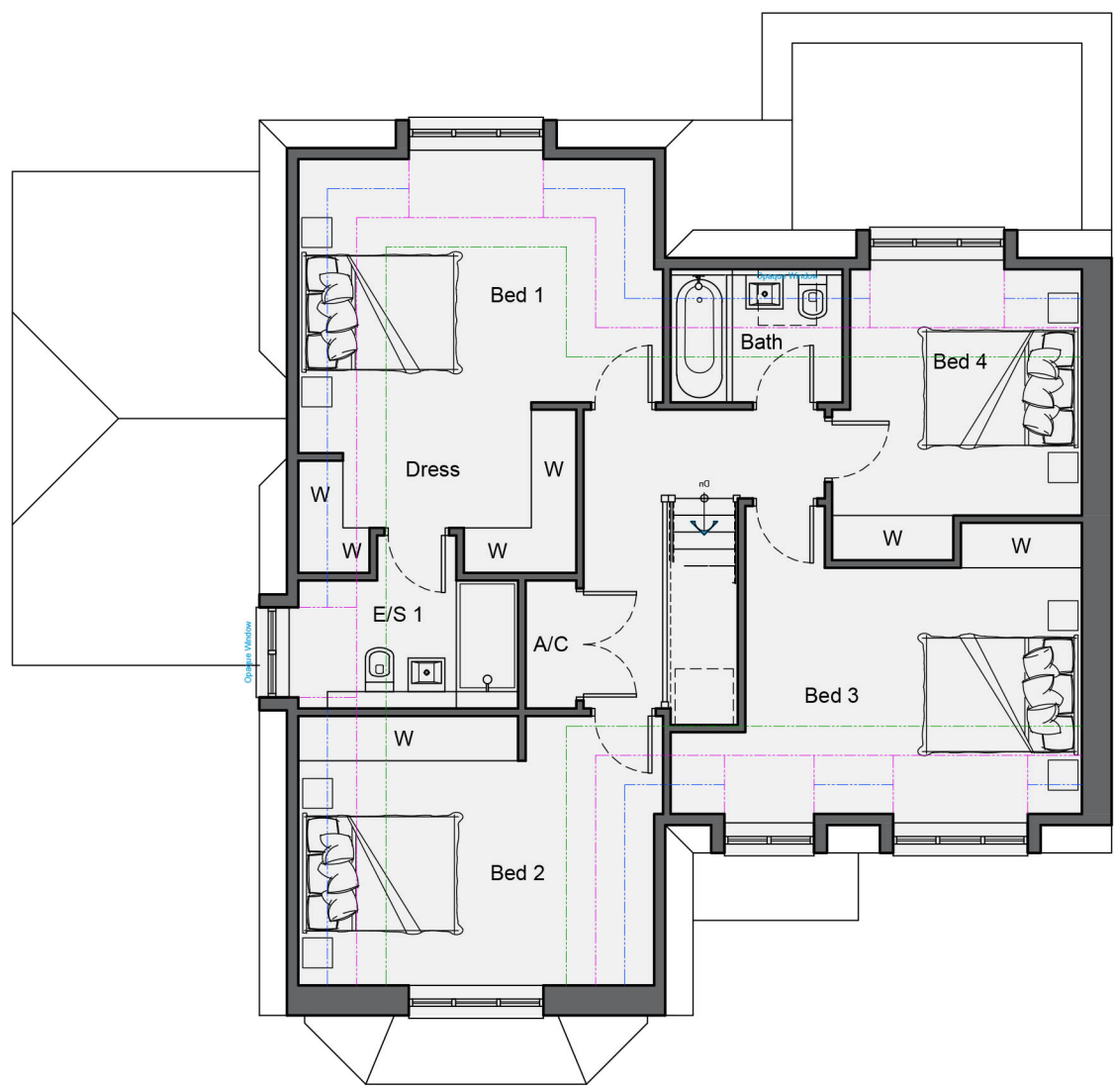
First Floor Plan GIA - 95.1m 2 (1,023ft 2 )
