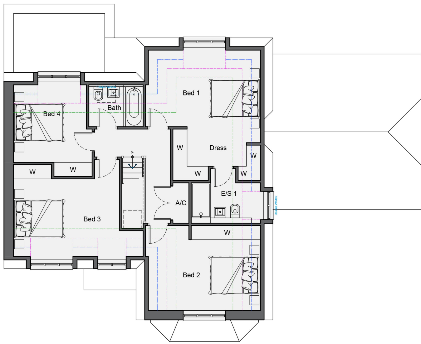
First Floor Plan GIA - 95.1m 2 (1,029ft 2 )
