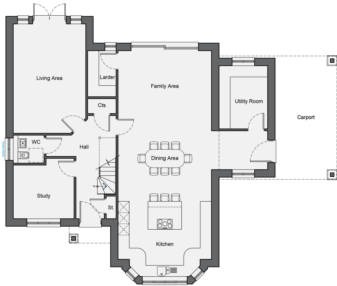
Ground Floor Plan GIA - 131.9m 2 (1,419ft 2 ) TOTAL GIA - 226.6m 2 (2,438ft 2 )
